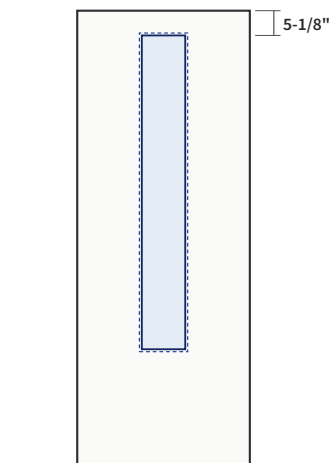
9" x 65" Full Sidelite, Wide Glass 8" x 64" Frame 10" x 66" Location 5-1/8" from top; 13-3/8" from each edge SKU ZCUT-GFS-0965
