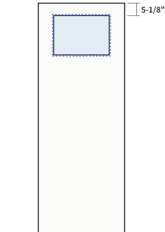
23" x 16-1/4" Craftsman, Short Glass 22" x 15-1/4" Frame 24" x 17.25" Location 5-1/8" from top; 6-3/8" from each edge SKU ZCUT-GCR-2316
