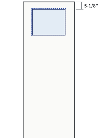
23" x 18" Craftsman Glass 22" x 17" Frame 24" x 19" Location 5-1/8" from top; 6-3/8" from each edge SKU ZCUT-GCR-2318
