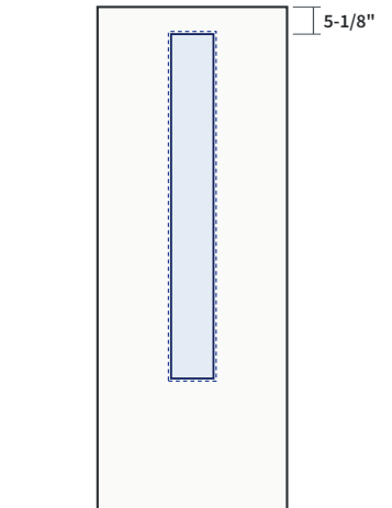
8" x 65" Full Sidelite Glass 7" x 64" Frame 9" x 66" Location 5-1/8" from top; 13-7/8" from each edge SKU ZCUT-GFS-0865
