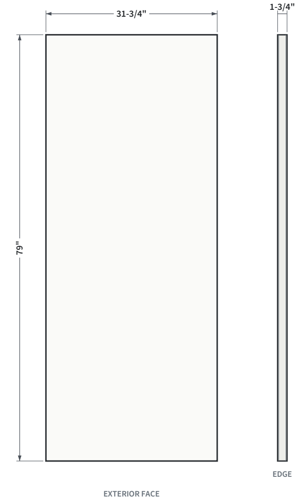
FIG. 1 ELEVATION AND EDGE VIEW Exterior face shown. Drawn to scale; dimensions are actual, in inches.
