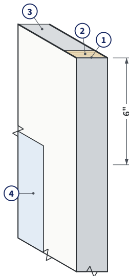
FIG. 2 CONSTRUCTION DETAIL
