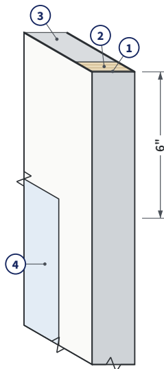
FIG. 2 CONSTRUCTION DETAIL
