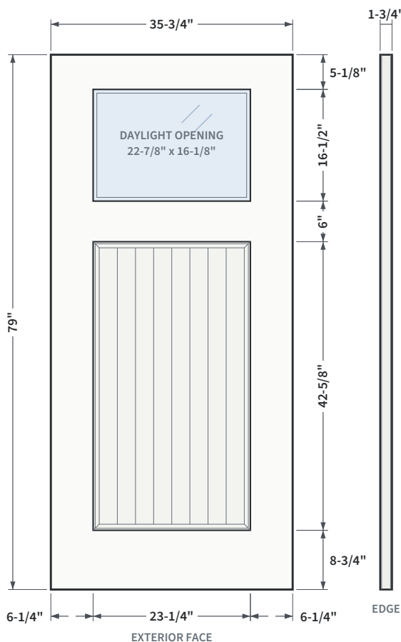
FIG. 2 PLANK PANEL PROFILE
