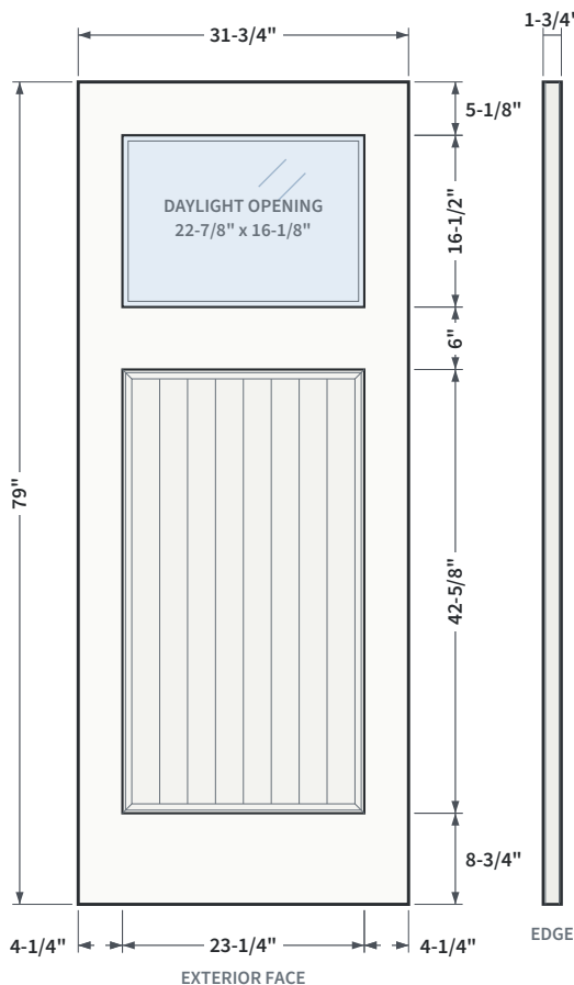
FIG. 2 PLANK PANEL PROFILE
