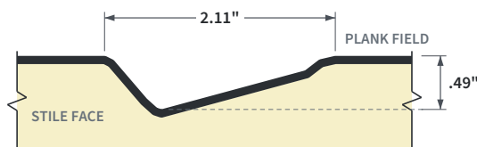
FIG. 2 PLANK PANEL PROFILE
