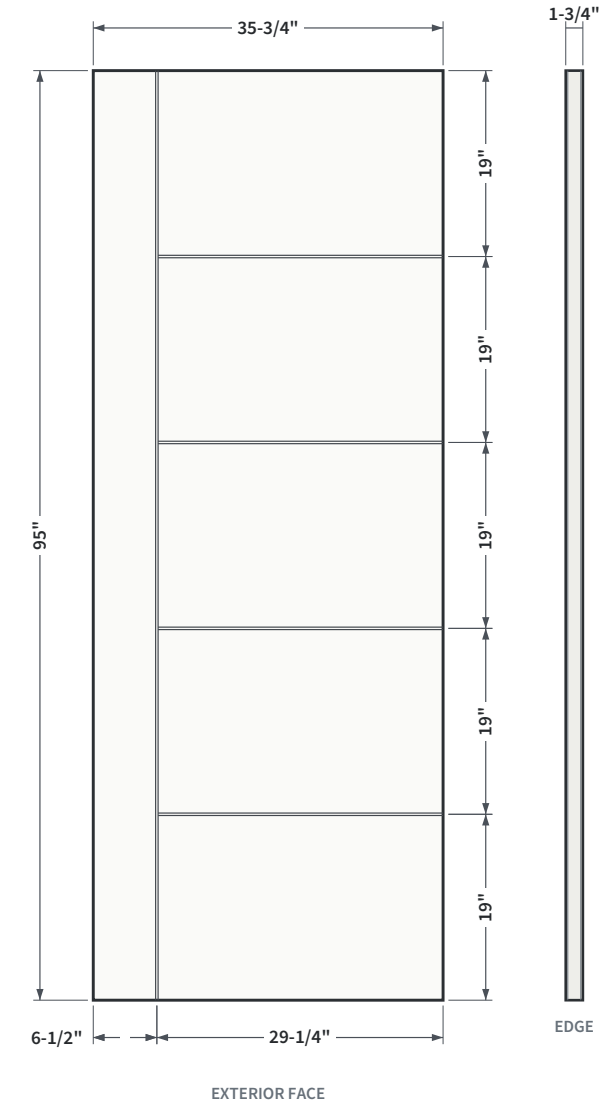
FIG. 1 ELEVATION AND EDGE VIEW Exterior face shown. Drawn to scale; dimensions are actual, in inches.
