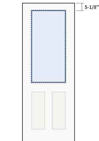
23" x 49" 3/4 Lite Glass 22" x 48" Frame 24" x 50" Location 5-1/8" from top; 6-3/8" from each edge SKU ZCUT-G34-2349
