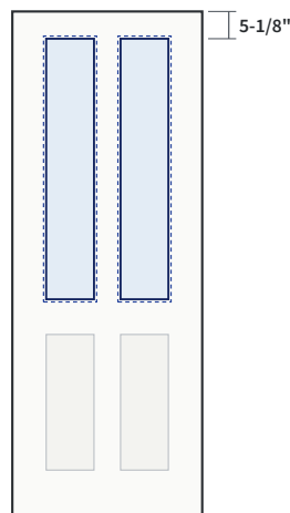
(2) 9" x 49" Tall Quarterlites (pair) Glass (2) 8" x 48" Frame 10" x 50" each Location 5-1/8" from top; one over each panel column, 5" apart SKU ZCUT-GH2-0949
