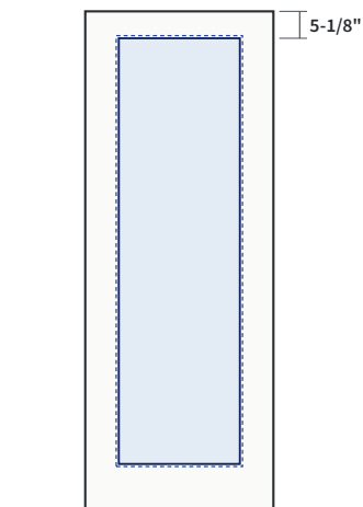
23" x 81" Tall Full Lite Glass 22" x 80" Frame 24" x 82" Location 5-1/8" from top; 6-3/8" from each edge SKU ZCUT-GFL-2381
