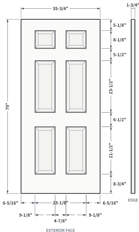
FIG. 2 RAISED PANEL PROFILE
