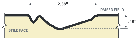
FIG. 2 RAISED PANEL PROFILE
