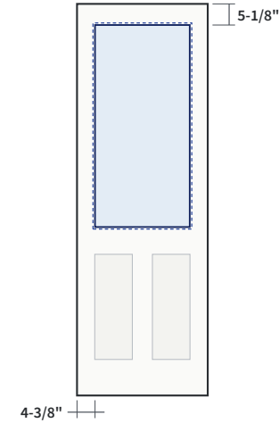
23" x 49" 3/4 Lite Glass 22" x 48" Frame 24" x 50" Location 5-1/8" from top; 4-3/8" from each edge SKU ZCUT-G34-2349
