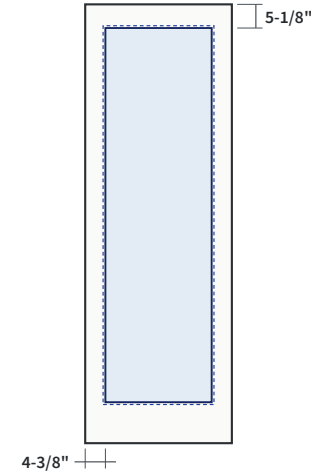
23" x 81" Tall Full Lite Glass 22" x 80" Frame 24" x 82" Location 5-1/8" from top; 4-3/8" from each edge SKU ZCUT-GFL-2381
