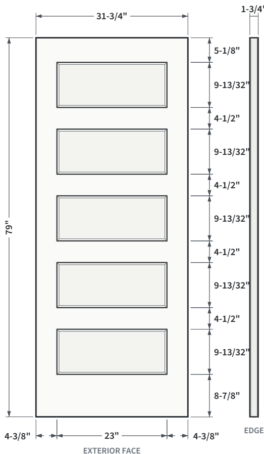
FIG. 2 SHAKER EMBOSSMENT PROFILE
