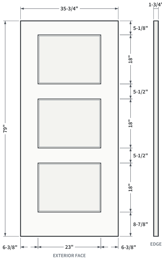
FIG. 2 SHAKER EMBOSSMENT PROFILE
