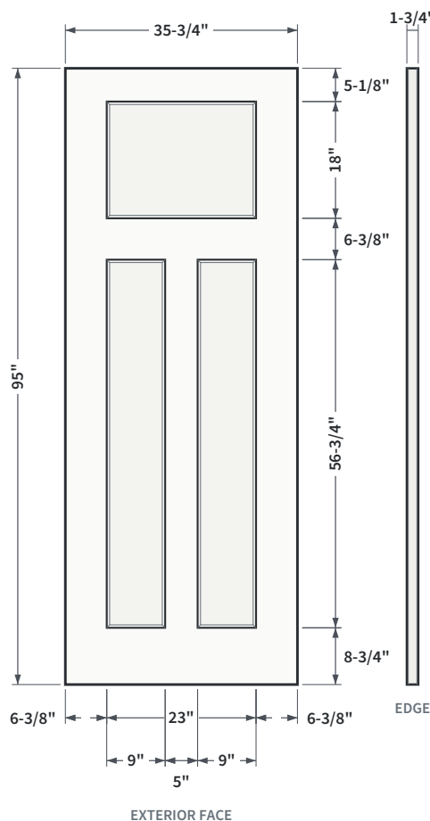
FIG. 2 SHAKER EMBOSMENT PROFILE
