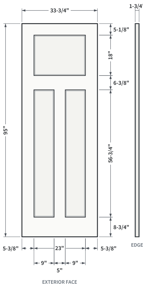
FIG. 2 SHAKER EMBOSMENT PROFILE
