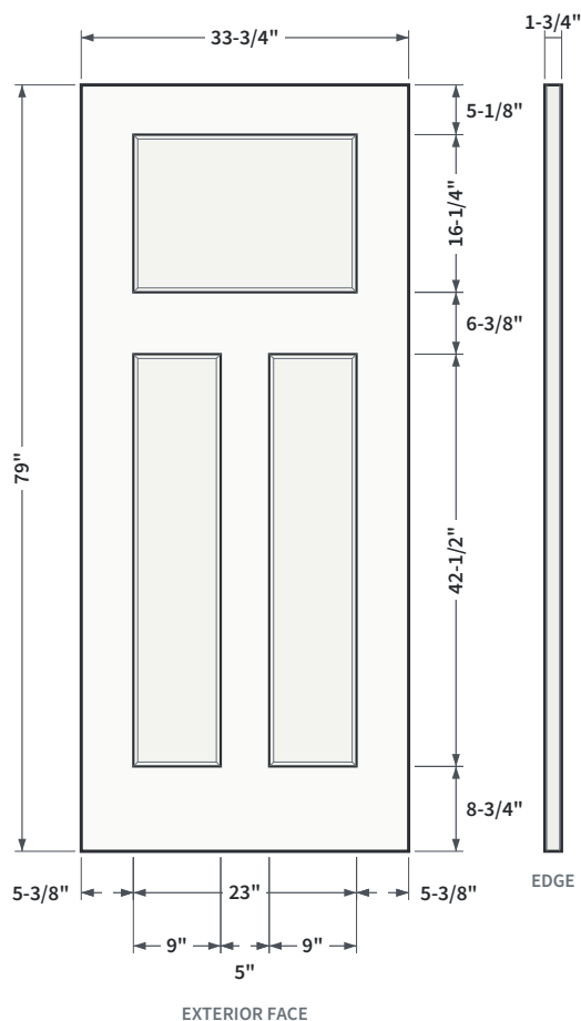
FIG. 2 SHAKER EMBOSMENT PROFILE
