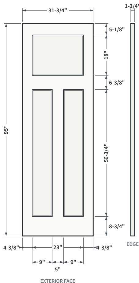
FIG. 2 SHAKER EMBOSMENT PROFILE
