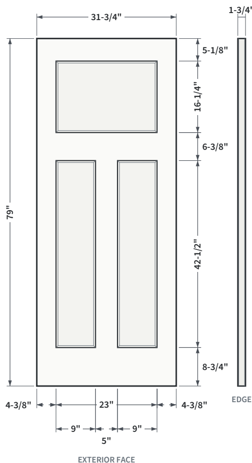
FIG. 2 SHAKER EMBOSMENT PROFILE
