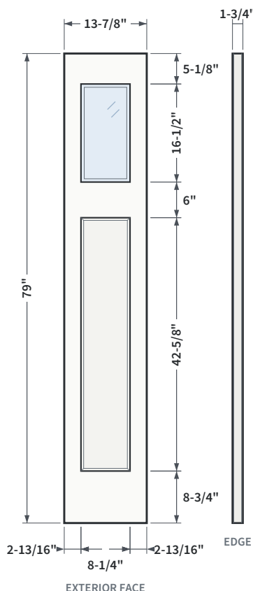
FIG. 2 SHAKER EMBOSSMENT PROFILE
