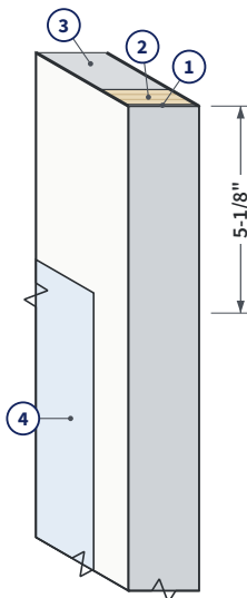
FIG. 3 CONSTRUCTION DETAIL
