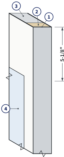
FIG. 3 CONSTRUCTION DETAIL Cutaway at the top corner
