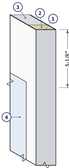
FIG. 3 CONSTRUCTION DETAIL
