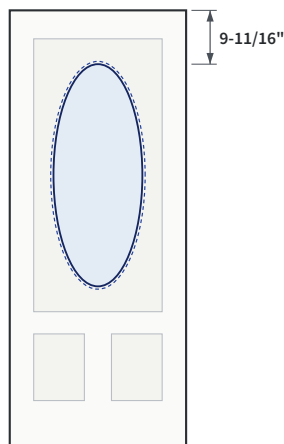
7-7/8" | 16" x 40" Medium Oval Glass 15-1/2" x 39-3/8" oval Frame 17.5" x 41.4" Location 9-11/16" from top; centered in the upper panel SKU ZCUT-VAL-MD
