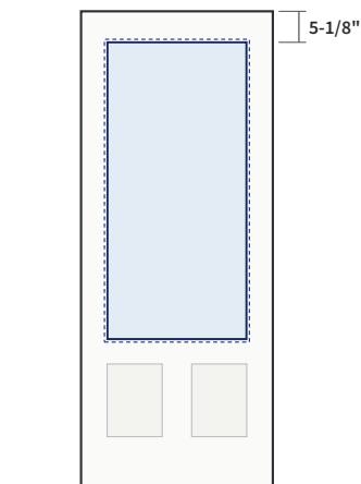
4-3/8" | 23" x 49" 3/4 Lite Glass 22" x 48" Frame 24" x 50" Location 5-1/8" from top; 4-3/8" from each edge SKU ZCUT-G34-2349
