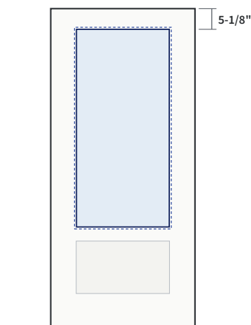
23" x 49" 3/4 Lite Glass 22" x 48" Frame 24" x 50" Location 5-1/8" from top; 6-3/8" from each edge SKU ZCUT-G34-2349
