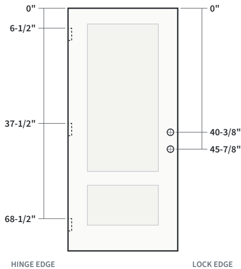
FIG. 2 LOCATIONS
