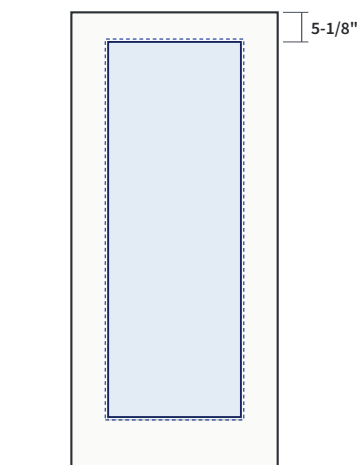
23" x 65" Full Lite Glass 22" x 64" Frame 24" x 66" Location 5-1/8" from top; 6-3/8" from each edge SKU ZCUT-GFL-2365
