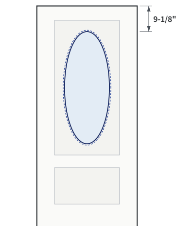
16" x 40" Medium Oval Glass 15-1/2" x 39-3/8" oval Frame 17.5" x 41.4" Location 9-1/8" from top; centered in the upper panel SKU ZCUT-VAL-MD
