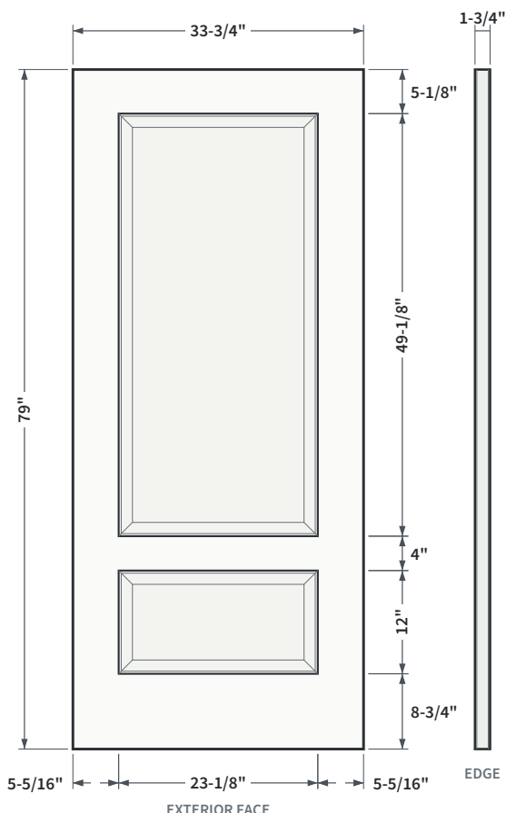
FIG. 2 RAISED PANEL PROFILE
