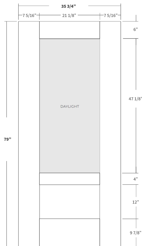
Fig. 1 — Slab elevation with daylight
