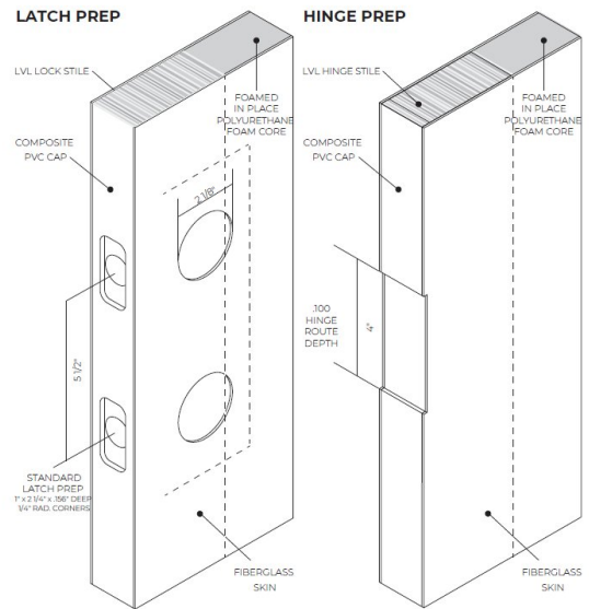
Fig. 3 — Latch & hinge stile cross-section
